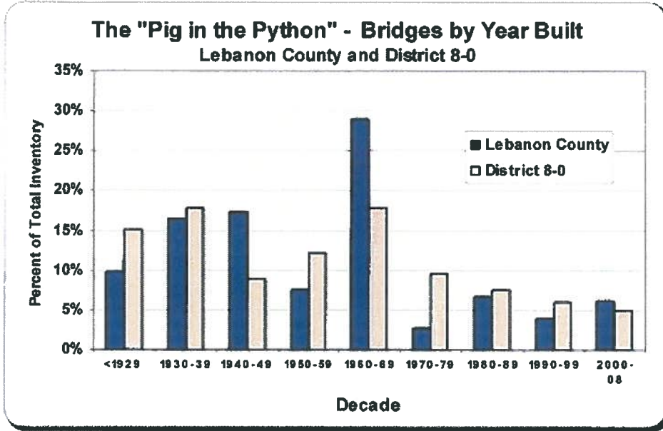
Figure 1 – Bridge Inventory by Year Built
